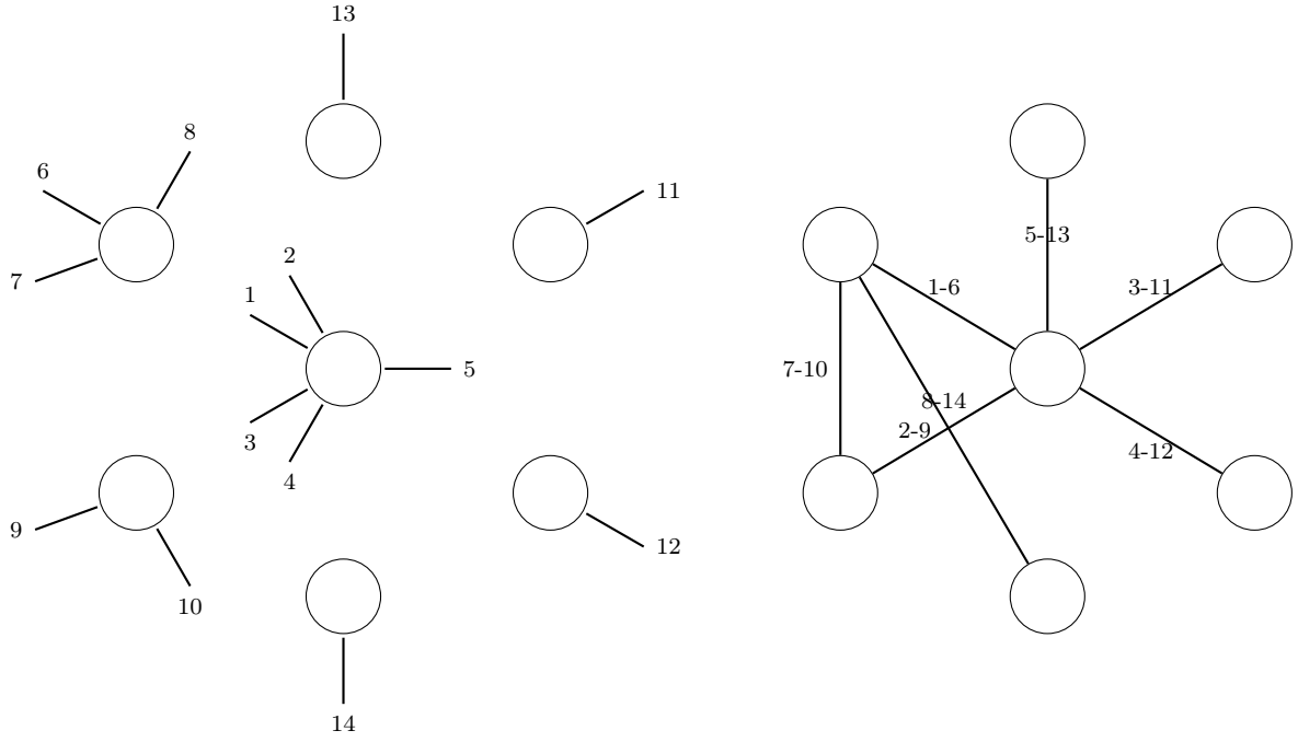
(a) Stubs generated from a scale-free degree sequence (b) Stubs paired into a simple realized graph
